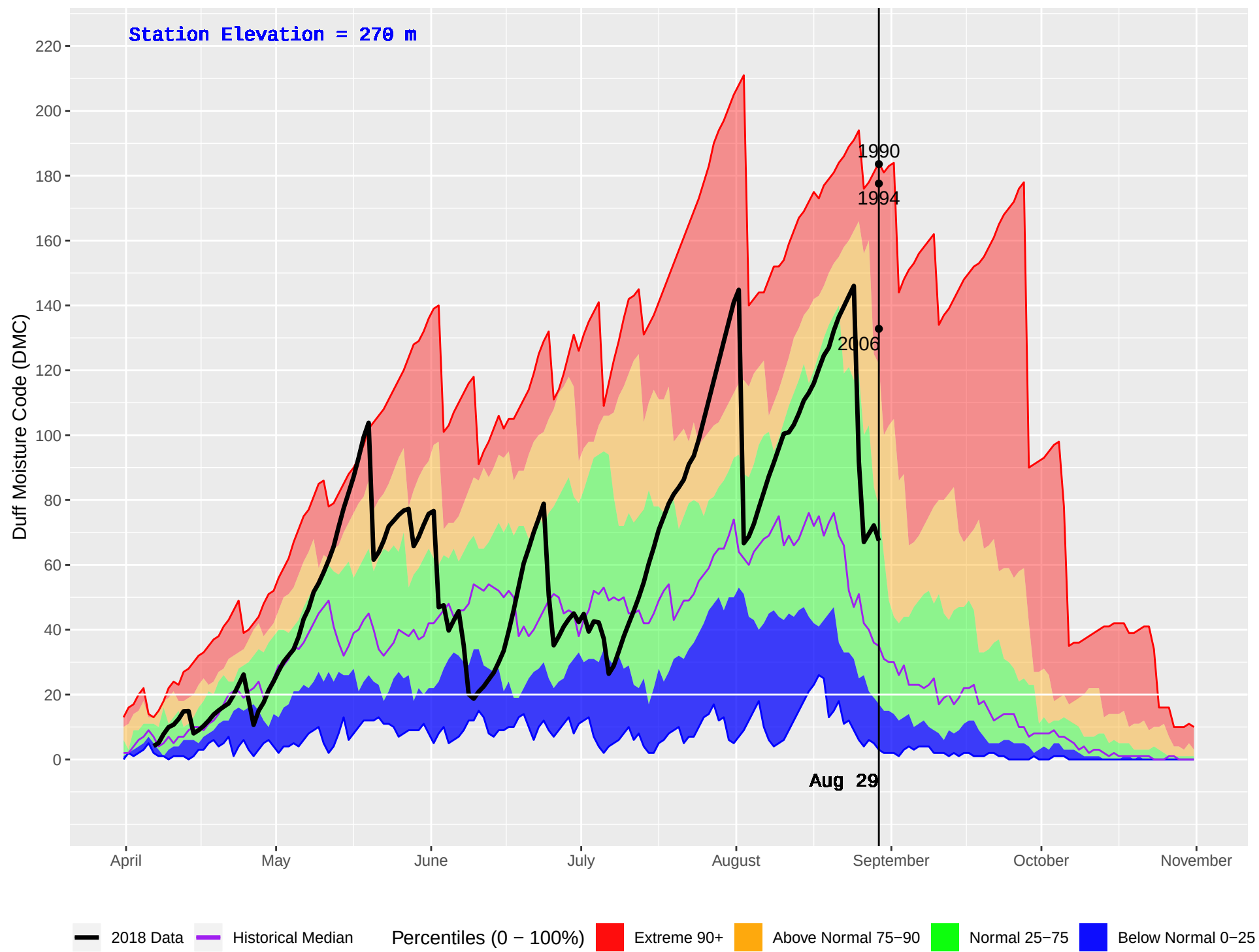
TALCHAKO (233) : Historical (1990–2016) and Current (2018) Daily Duff Moisture Code (DMC)
