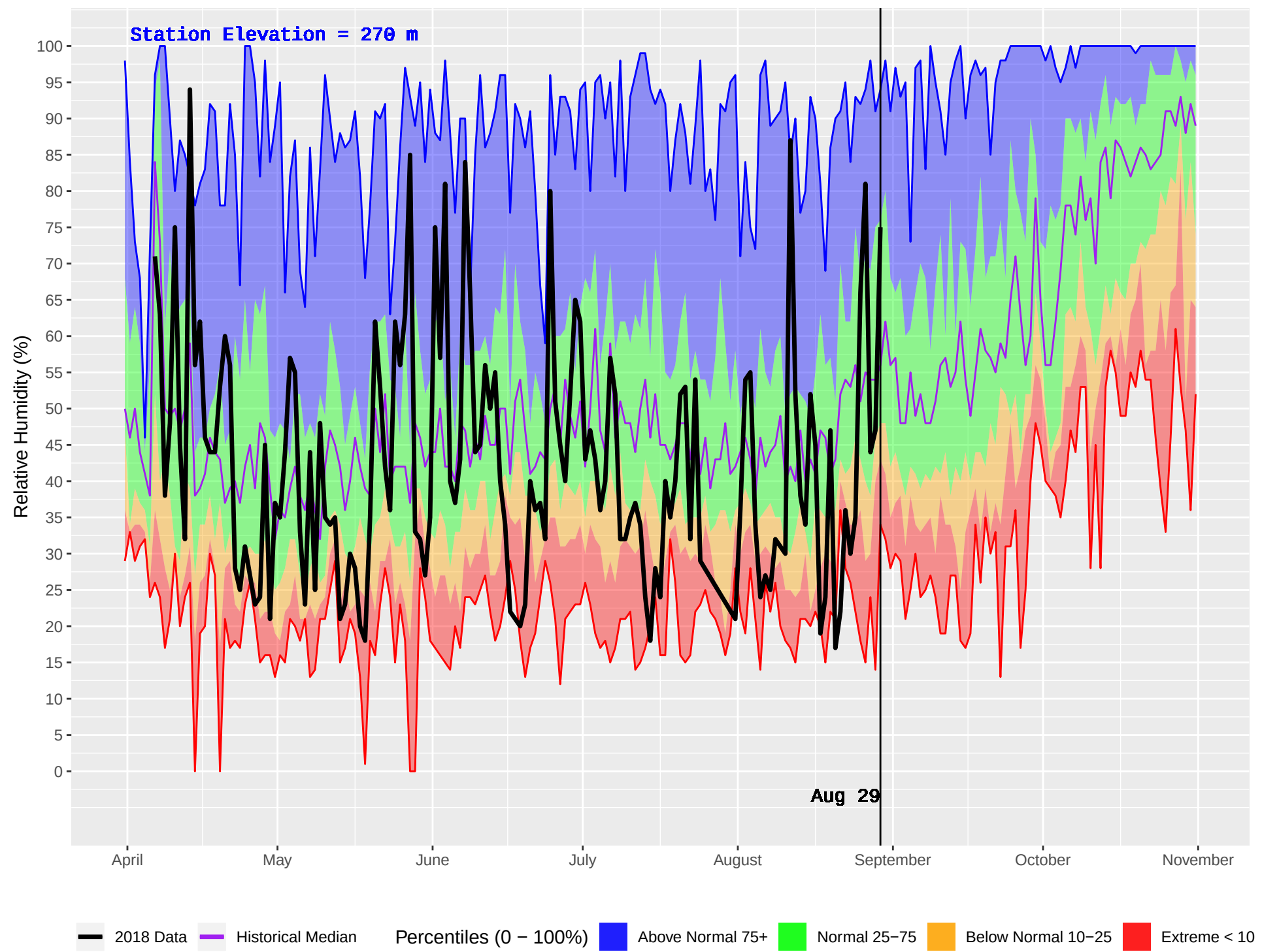
TALCHAKO (233) : Historical (1990–2016) and Current (2018) Daily Relative Humidity
