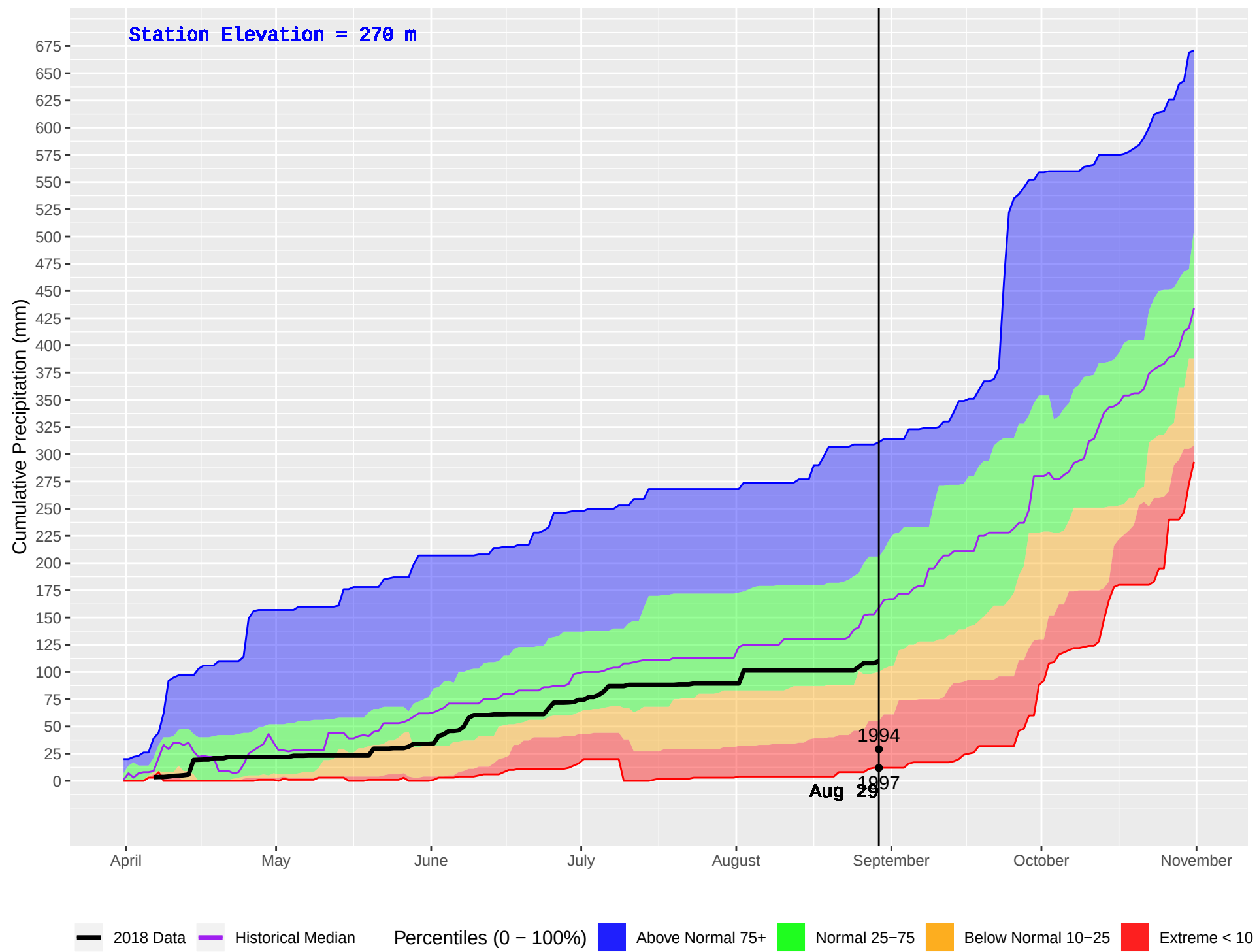
TALCHAKO (233) : Historical (1990–2016) and Current (2018) Daily Cumulative Precipitation
