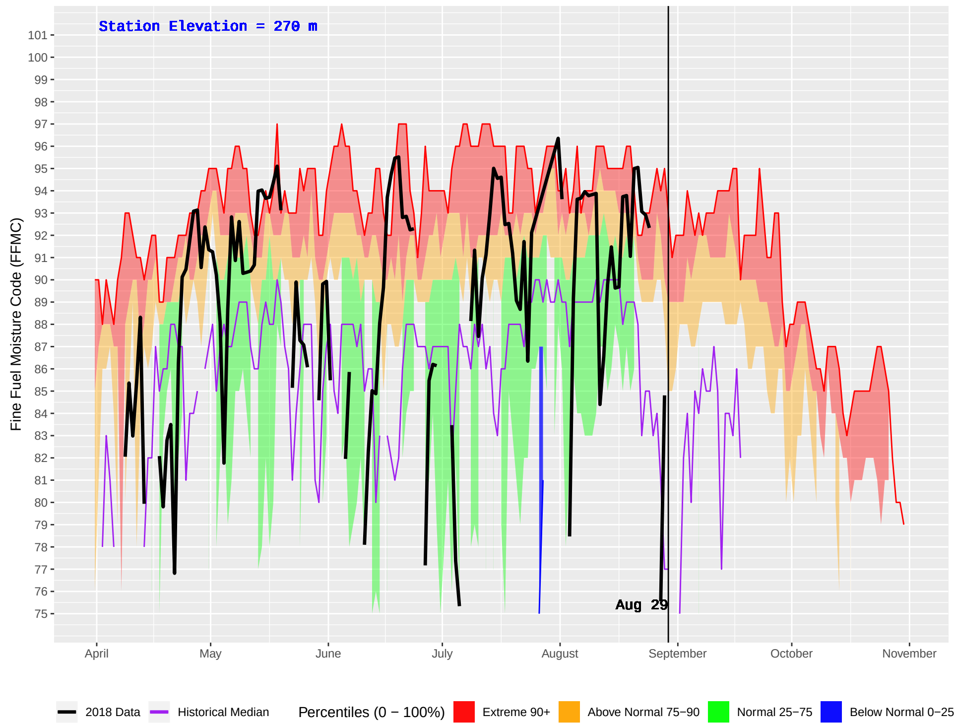
TALCHAKO (233) : Historical (1990–2016) and Current (2018) Daily Fine Fuel Moisture Code (FFMC)
