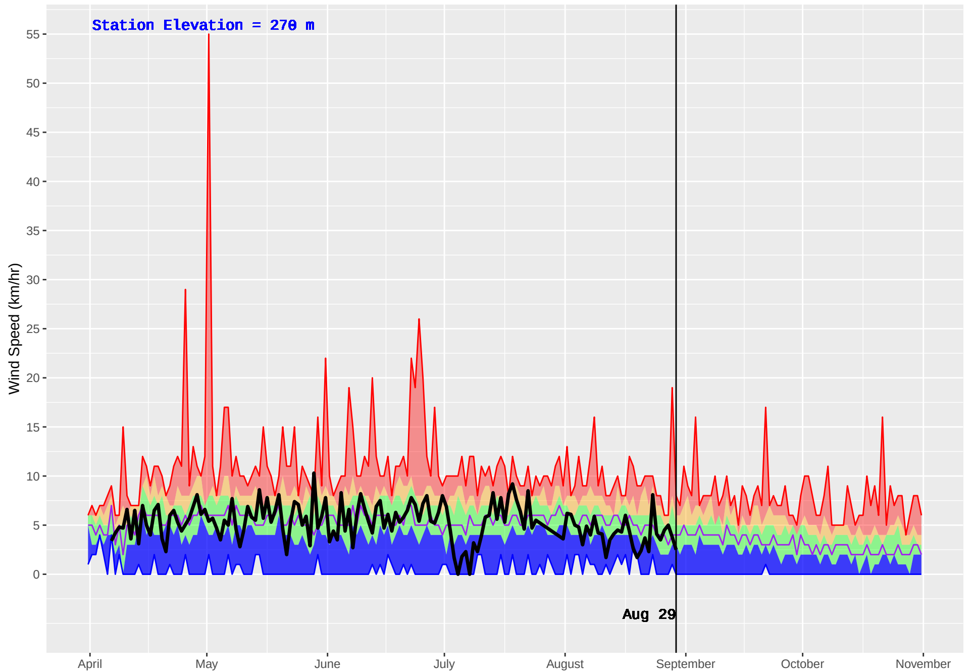
TALCHAKO (233) : Historical (1990–2016) and Current (2018) Daily Wind Speed
