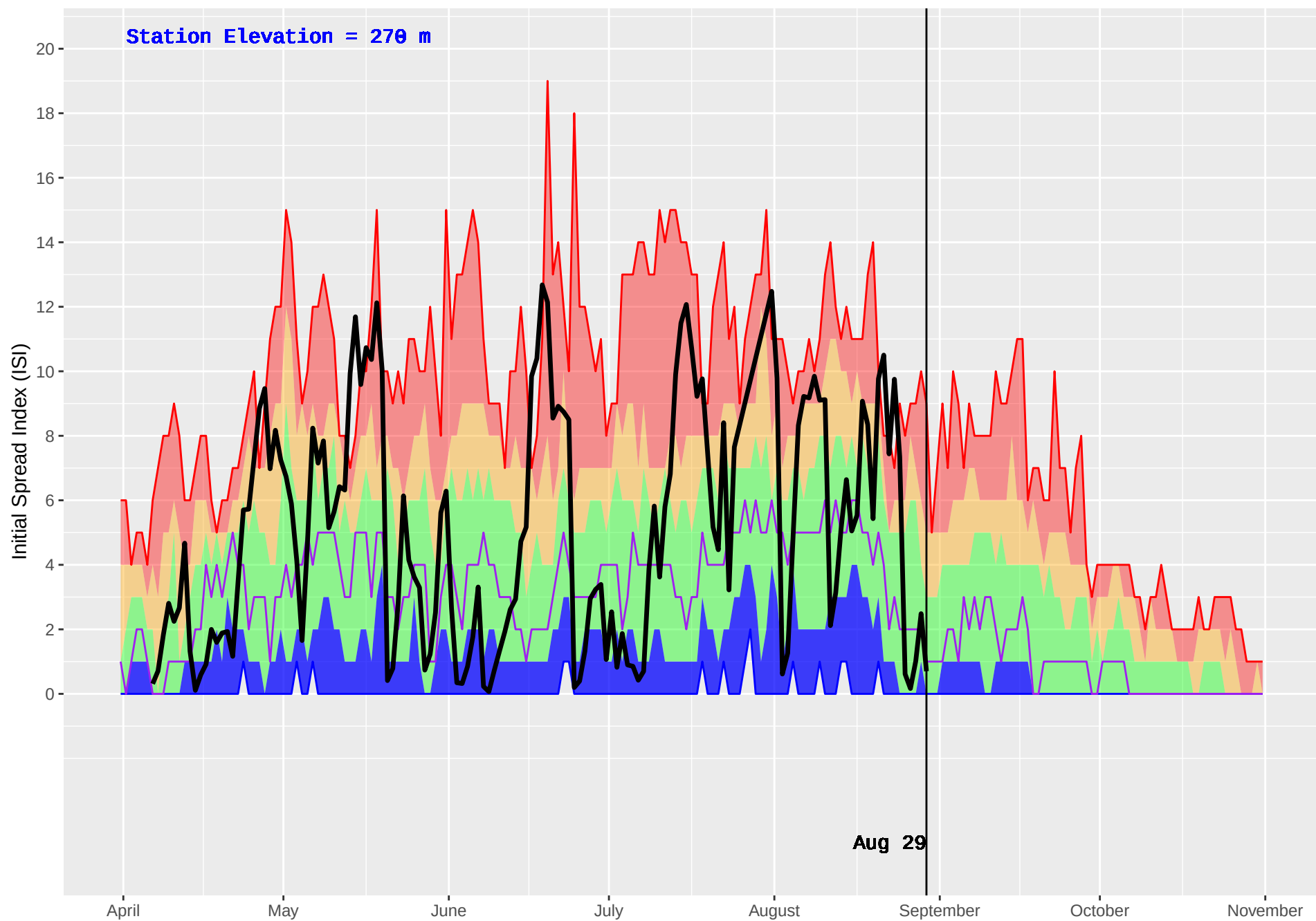
TALCHAKO (233) : Historical (1990–2016) and Current (2018) Daily Initial Spread Index (ISI)
