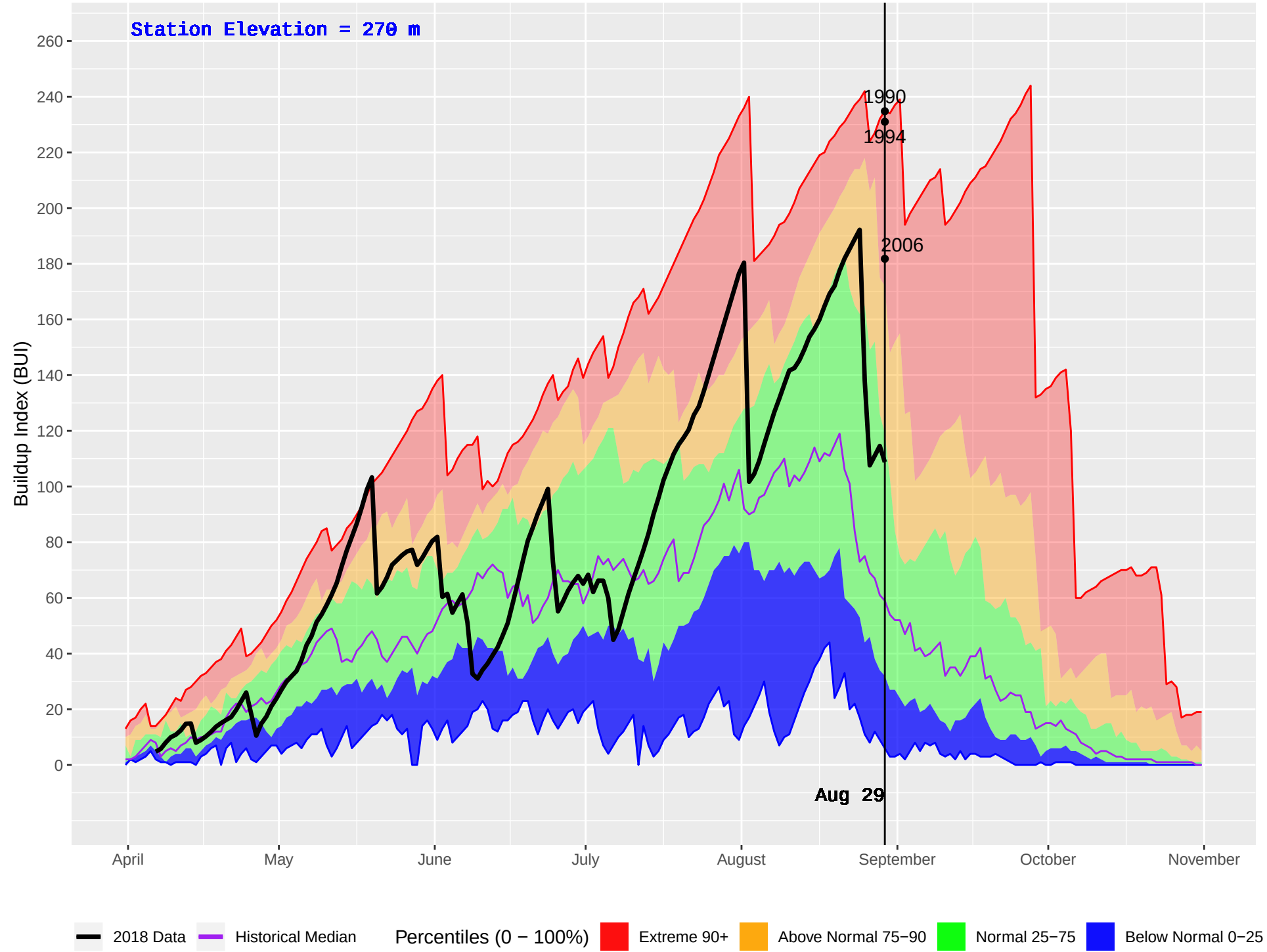
TALCHAKO (233) : Historical (1990–2016) and Current (2018) Daily Buildup Index (BUI)
