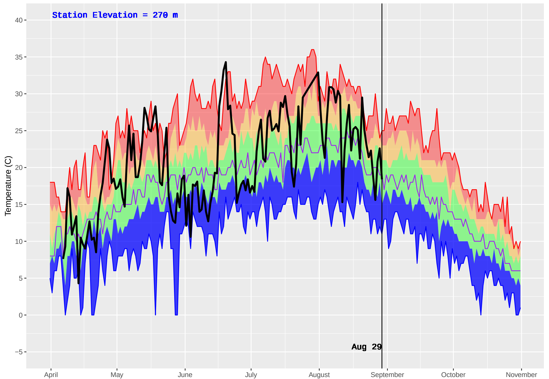
TALCHAKO (233) : Historical (1990–2016) and Current (2018) Daily Temperature
