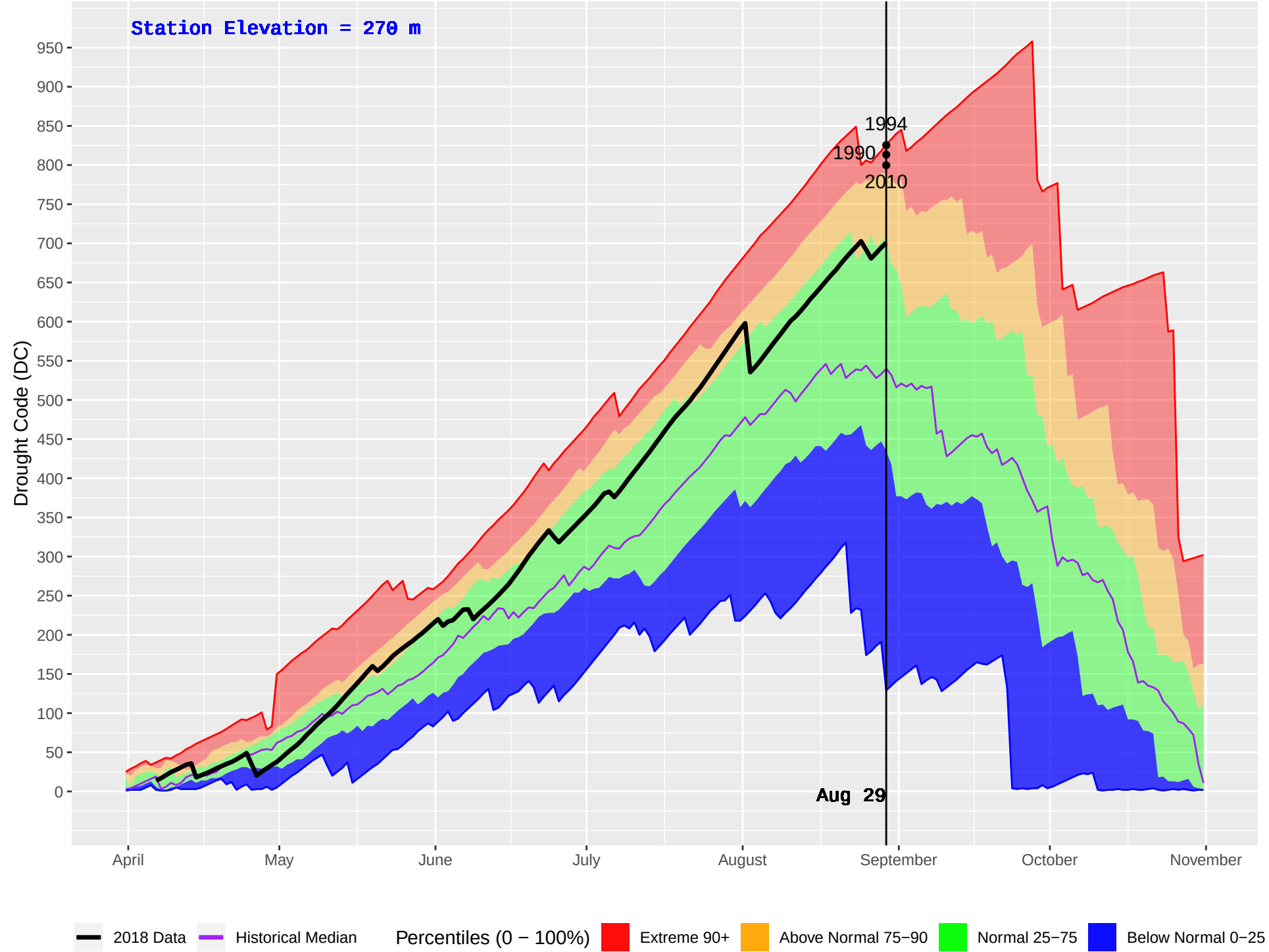
TALCHAKO (233) : Historical (1990–2016) and Current (2018) Daily Drought Code (DC)
